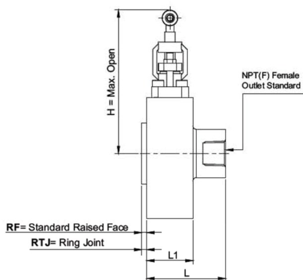
OS&Y Bonnet Dimensions (inches)
